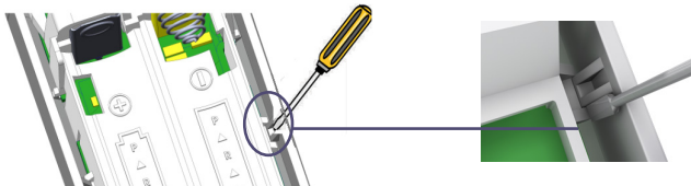
Figure 3 – Removing the Main Unit
