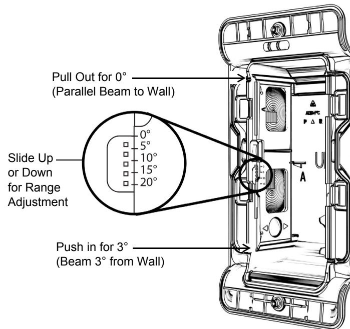
Figure 2 : Beam Adjustment
